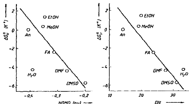
Fig. 3. Free enthalpies of transfer (acetonitrile as reference solvent) for K^+ versus the solvent HOMO eigenvalues and versus solvent donor number, respectively, in different solvents [53].
